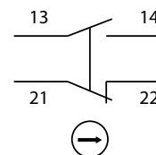
Wiring diagram of the switches PRSL0100XX
